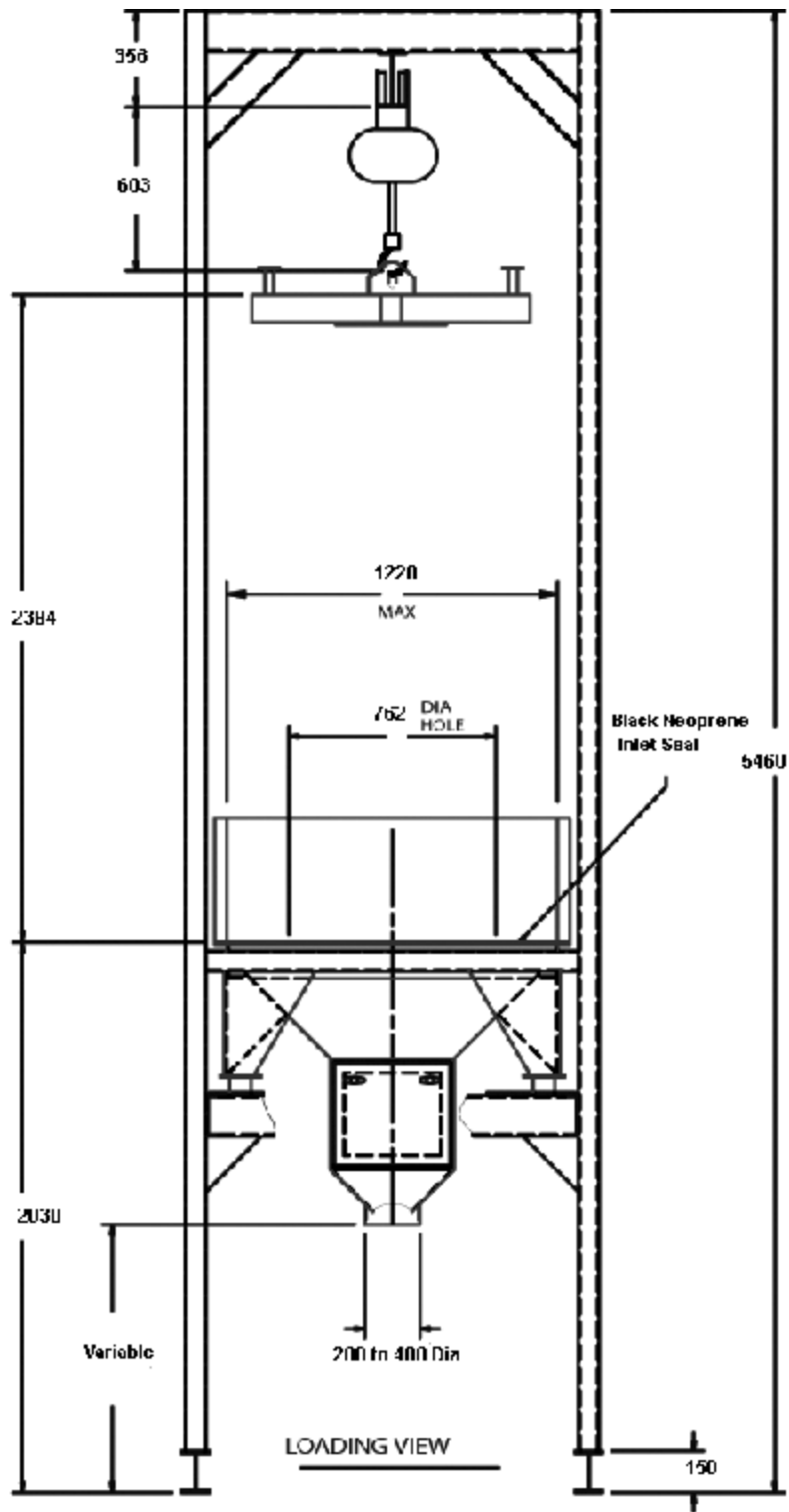
Discharger with Hoist
